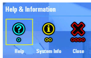
Figure 9. Help Menu
